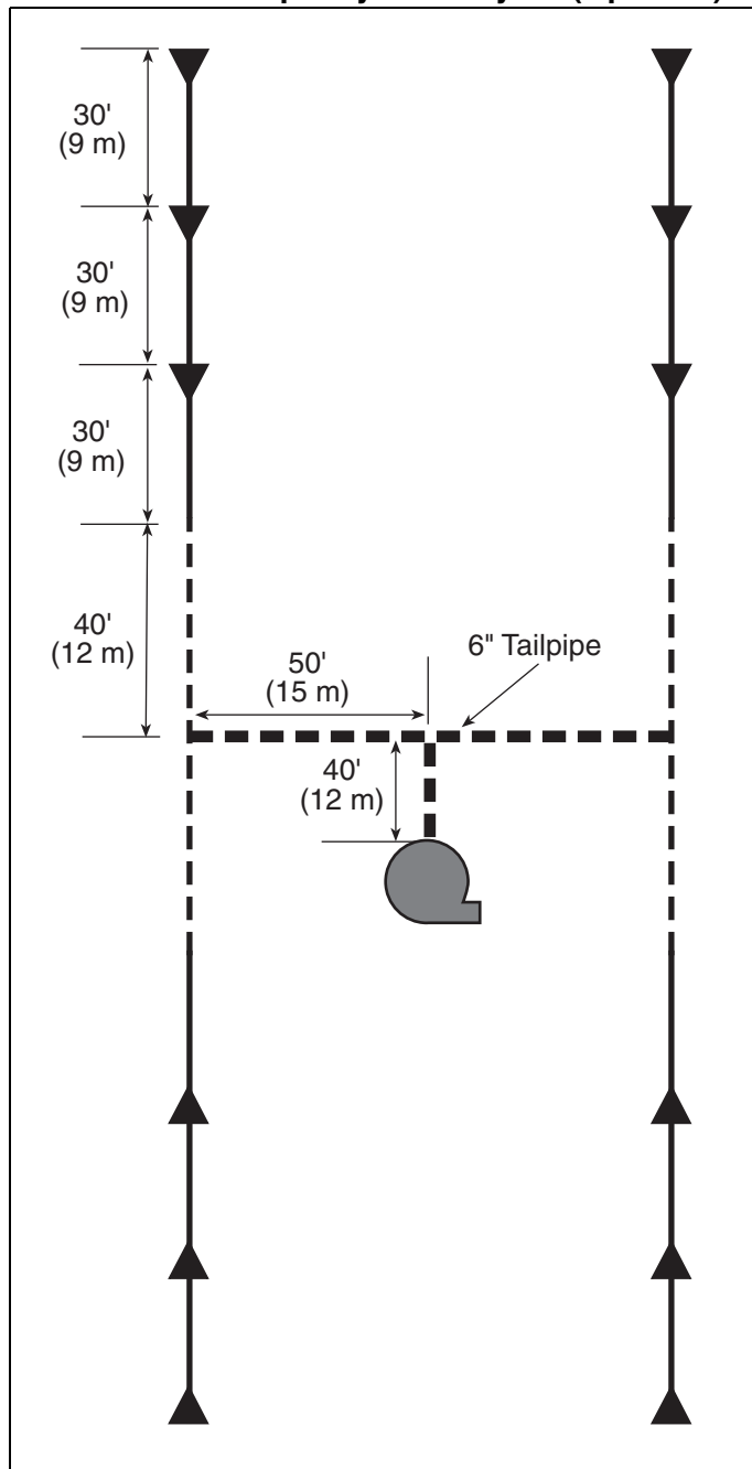
FIGURE 20: Example System Layout (Option 3)
